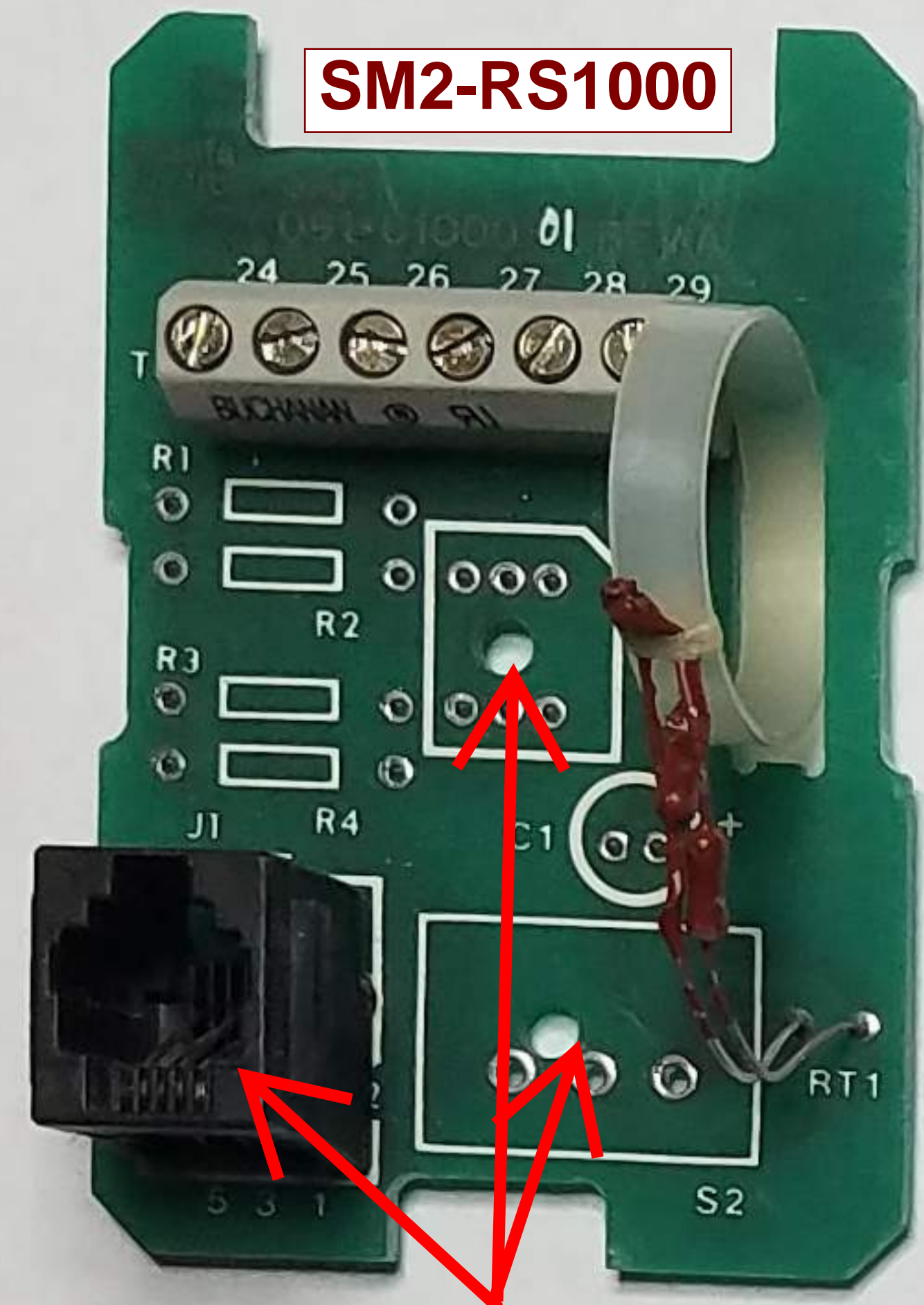
Very Old Style. Front Facing Service Tool Port No Setpoint. No Override.
